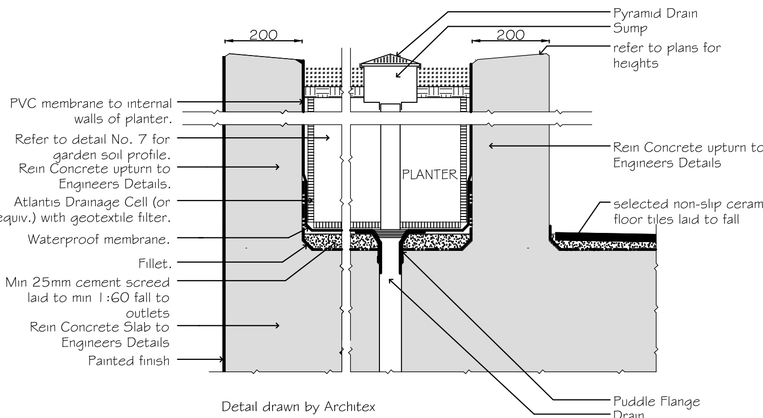
2 RAISED PLANTER BOX WALLS AND WATERPROOFING - ROOFTOP SCALE 1:10 TYPICAL SECTION.
