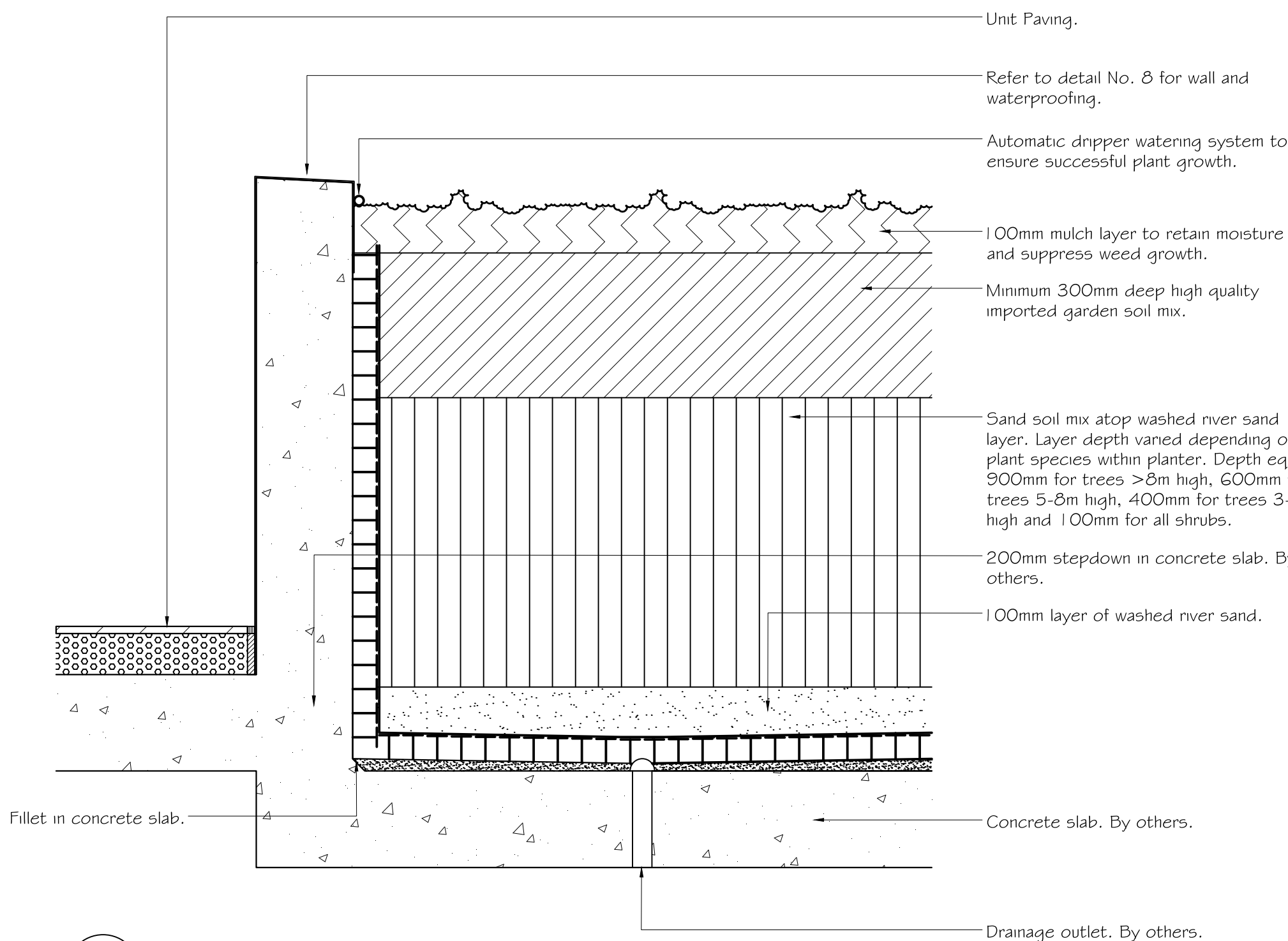
1 RAISED PLANTER BOX - ROOFTOP SCALE 1:10 TYPICAL SECTION.
